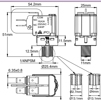
1/4" NPSM thread
